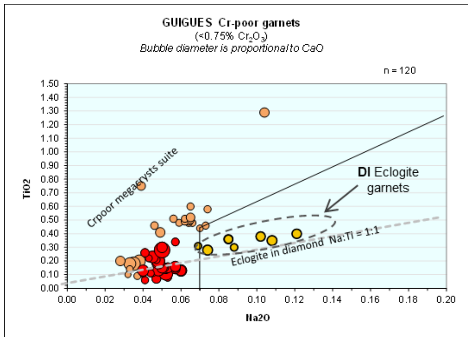
Figure 2: Low chromium garnets from Guigues, including those that plot in the eclogite diamond inclusion field.
